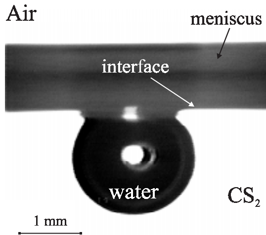
Fig. 3. Photograph of a water drop floating at the CS 2 surface.
