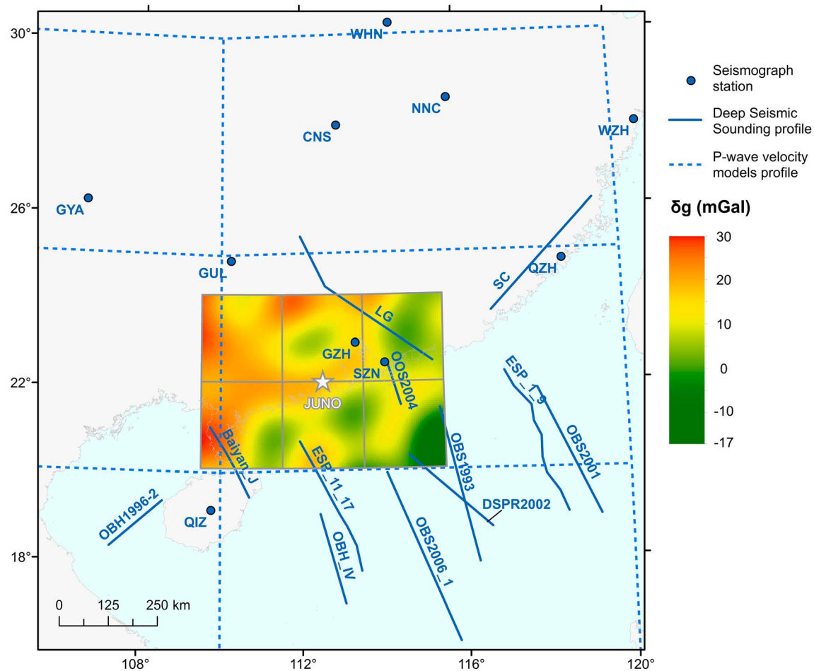
Figure 2. Geophysical input data used for the construction of the 3-D model in the 6^{\circ} \times 4^{\circ} area centered at the JUNO detector location ( 22^{\circ}07'05'' N, 112^{\circ}31'05'' E; An et al., 2016). Deep seismic sounding profiles, P wave velocity profiles, and locations of seismograph stations correspond to the input seismic data used to build the a priori model for the inversion of gravimetric data. The raw observations of gravimetric disturbances ( \delta g ) are represented as a continuous grid with 5 \text{ km} \times 5 \text{ km} resolution. JUNO = Jiangmen Underground Neutrino Observatory.
