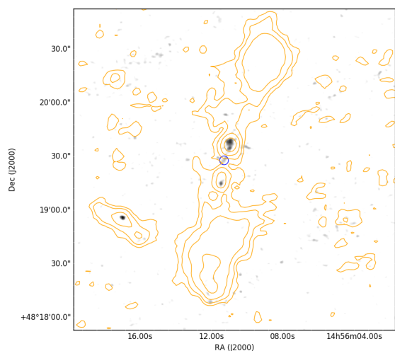
A.1. 36 ILTJ145610.69+481923.0 ROBUST: 0.5
