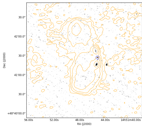
A.1. 34 ILTJ145147.28+484123.5 ROBUST: -0.5
