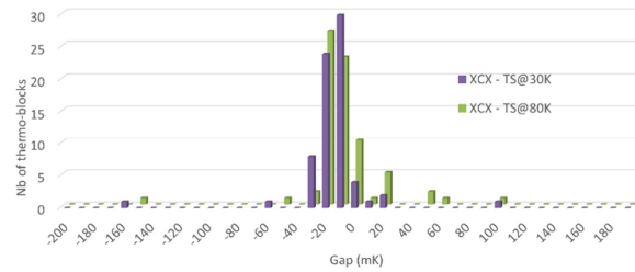
Fig. 12: Gap @4.2K between measured and reference temperature for two thermal shield temperatures and for un-calibrated CERNOX TM sensors (ref. XCX-1050-SD-HT-376).
