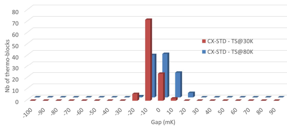
Fig. 11: Gap @4.2K between measured and reference temperature for two thermal shield temperatures and for calibrated CERNOX TM sensors (ref. CX-1050-SD-HT-1.4L).
