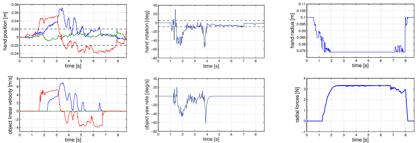
(a) Top: displacement vector o_h of the position of the hand centroid with respect to the rest position (blue \rightarrow x , green \rightarrow y , red \rightarrow z ). Horizontal dashed black lines are used to delimitate the dead zone. Bottom: velocity of the centroid of the teleoperated box.
