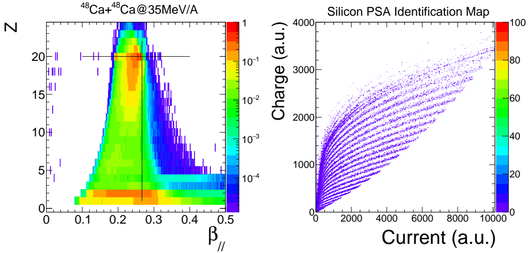
Fig. 3. – Left : two dimensional plot of the correlation between the charge ( Z ) and the parallel velocity ( \beta_{//} in c units) of fragments identified in Si-Si and Si-CsI telescopes. Right : typical identification map obtained using the correlation between the maximum of charge signal and the maximum of current signal for nuclei stopped in the first silicon detector.
