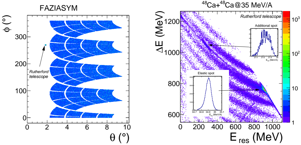
Fig. 1. – Left : angular coverage of the FAZIASYM set-up. The "Ruth-Tel" indicated the position of the Si-Si telescope dedicated to a continuous monitoring of the Rutherford elastic scattering during beam time. Right : \Delta E - E_{res} identification map of the "Rutherford" telescope around the elastic scattering region. The two insets show the total energy per nucleon of the two main spots : the expected one localized close to the initial beam energy (34.9 MeV/A) and a second one at 27.6 MeV/A.
