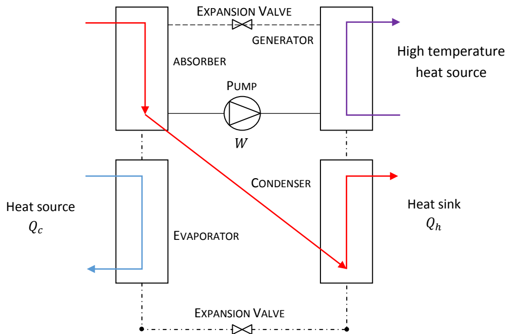
Figure 11: Absorption system cycle
