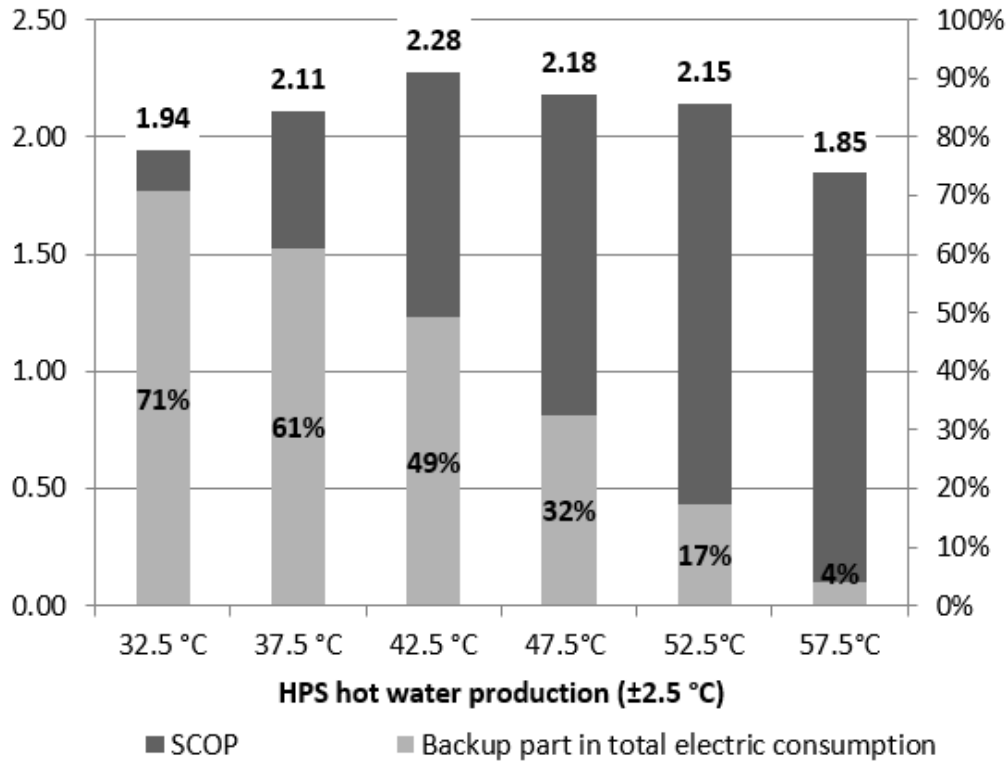
Figure 8: Impact of hot water production temperature on SCOP for a residential low-energy building [5]
