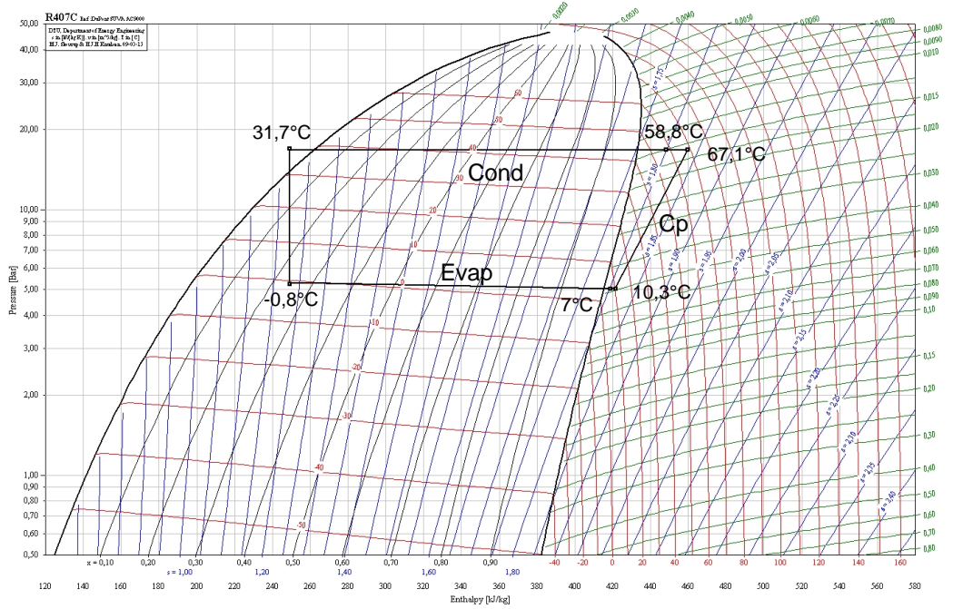
Figure 7: Thermodynamic cycle drawn with experimental measurements during a simultaneous mode [20]
