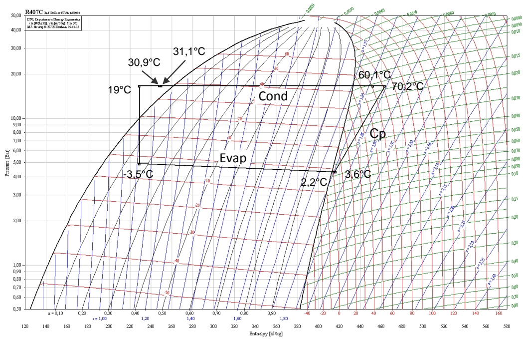
Figure 6: Thermodynamic cycle drawn with experimental measurements during a heating mode [20]
