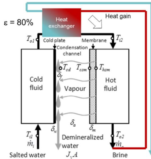
Figure 9: Scheme of air gap membrane distillation system [30]
