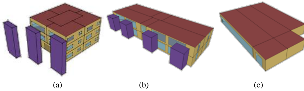
Figure 1. 3D view of residential building (a), office building (b) and retail store (c)
