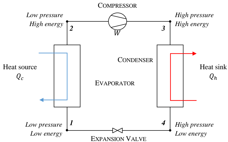
Figure 5: Vapour-compression cycle [14]
