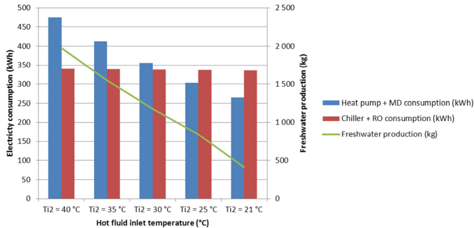
Figure 10: Comparison between a heat pump for simultaneous cooling and desalination and the association of a chiller and a reverse osmosis desalination system [30]
