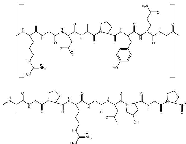
Figure 22: Top: one example of a repeated motif of an UCST polypeptide as designed by Chilkoti's group. The amino acid sequence is RGDAPYQG, repeated 28 times it gives a polypeptide with a critical temperature of 50 °C in PBS. Bottom: basic structure of the gelatin protein.
