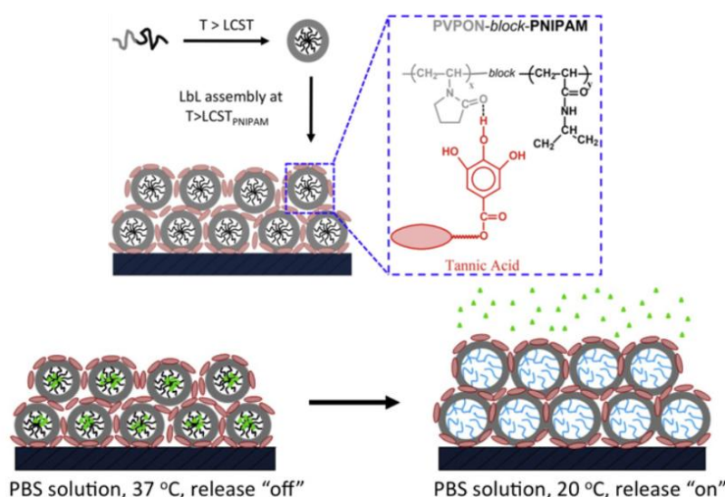
Figure 9: Schematic representation of a layer-by-layer film of thermoresponsive micelles loaded with doxorubicin at temperature higher than the LCST, 37 °C and the response after cooling at 20 °C. The inset shows the possible hydrogen bonding between tannic acid and the hydrophobic block PVPON.
