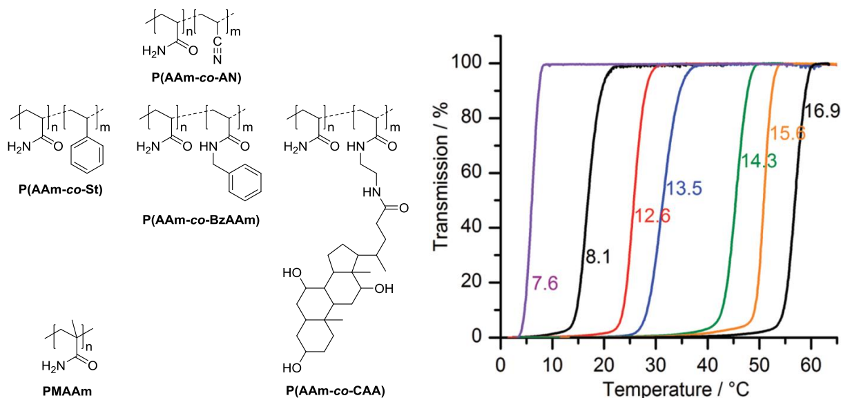
Figure 20: Left: chemical structure of acrylamide copolymers reported to have a UCST behavior in water. P(AAm-co-AN): poly(acrylamide-co-acrylonitrile); P(AAm-co-St): poly(acrylamide-co-styrene); P(AAm-co-BzAAm): poly(acrylamide-co-N-benzylacrylamide); P(AAm-co-CAA): poly(acrylamide-co-cholic acid acrylamide); PMAAm: poly(methacrylamide). Right: UV-vis transmittance cooling curves of P(AAm-co-AN) copolymers with different mol.% amounts of acrylonitrile, given by the numbers, from [114].
