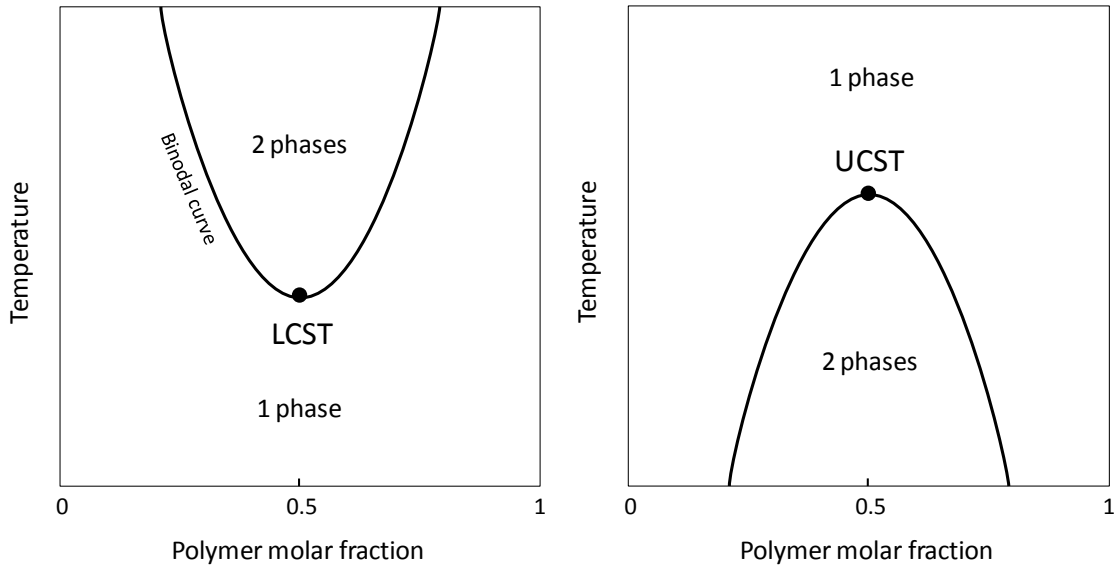
Figure 1: Simplified phase diagrams of thermoresponsive polymers. Outside the region delimited by the binodal curve, there is a homogeneous solution of solubilized polymer in aqueous solution (1 phase). Inside the region, the solution is not stable anymore and the polymer phases out (2 phases).
