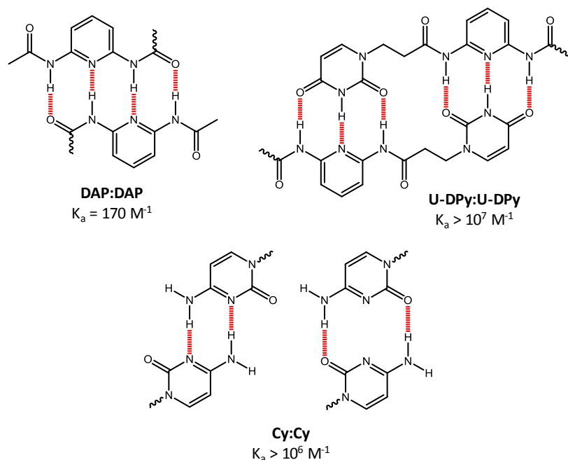
Figure 8: Chemical representation of potential hydrogen bond dimers studied. Hydrogen bonds represented in red, wavy bonds represent links to polymer, K_a is the association constant. DAP: diacylamido pyridine. U-DPy: N-(6-(3-(2,4-dioxo-3,4-dihydropyrimidin-1(2H)-yl)propanamido)pyridin-2-yl)undec-10-enamide. Cy: cytosine. Adapted from [67][68].
