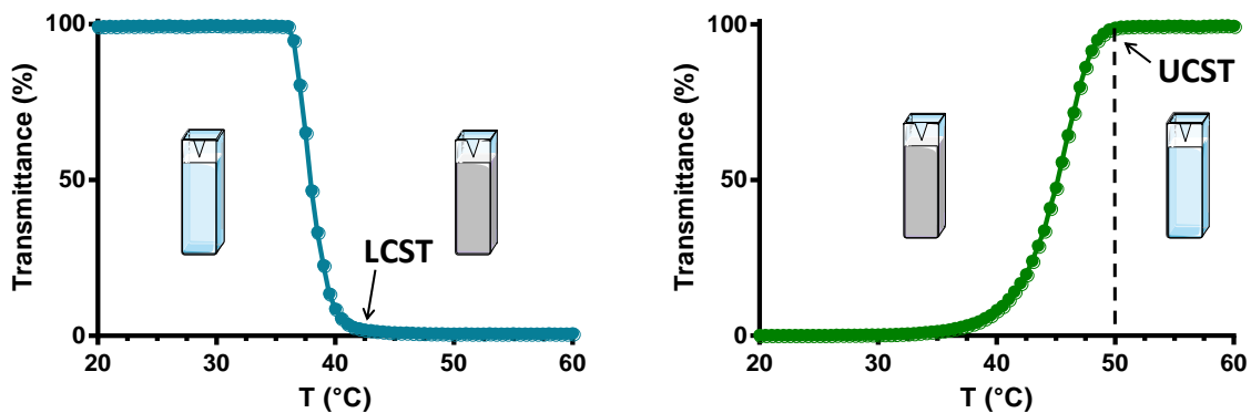
Figure 2: Model transmittance curves as a function of temperature for LCST (left) and UCST (right) polymers. When transmittance is at 100%, the sample is completely transparent and there are no apparent particles in solution. When transmittance is close to 0%, the sample appears turbid due to the presence of particles. In this case, the depicted LCST corresponds to 42.5 °C, and the UCST 50 °C.
