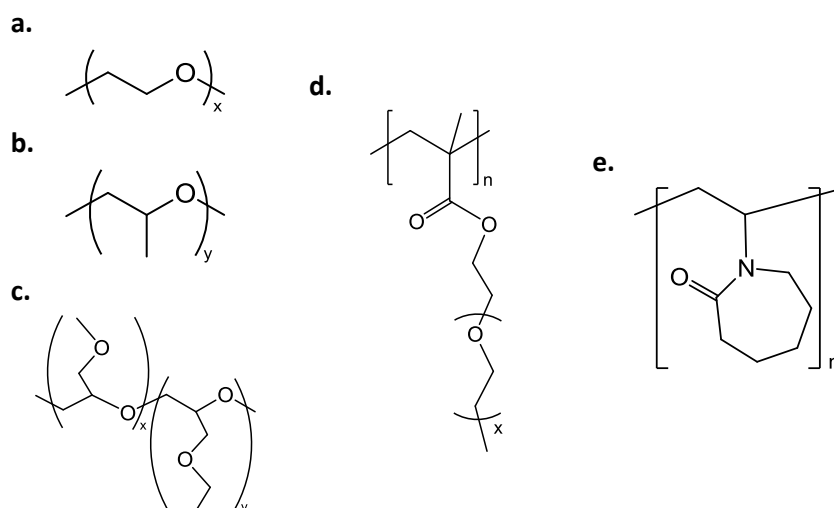
Figure 6: Chemical structure of other LCST polymers used for nanocarrier fabrication. a: poly(ethylene glycol) (PEG), b: poly(propylene glycol) (PPG), c: poly(glycidyl methyl ether-co-glycidyl ethyl ether) (P(GME-co-GEE)), d: poly(oligoethylene glycol) methyl ether methacrylate (POEGMA), e: poly(N-vinylcaprolactam) (PNVCL).
