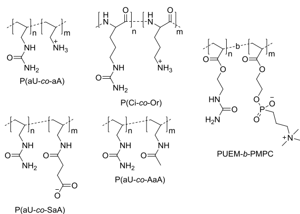
Figure 21: Chemical structure of ureido-bearing polymers reported to have a UCST behavior in aqueous solution. P(aU-co-aA): poly(allylurea-co-allylamine); P(Ci-co-Or): poly(citrulline-co-ornithine); P(aU-co-SaA): poly(allylurea-co-succinylated allylamine); P(aU-co-AaA): poly(allylurea-co-acetylated allylamine); PUEM-b-PMPC: poly(2-ureidoethylmethacrylate)-b-poly(2-methacryloyloxyethyl phosphorylcholine).
