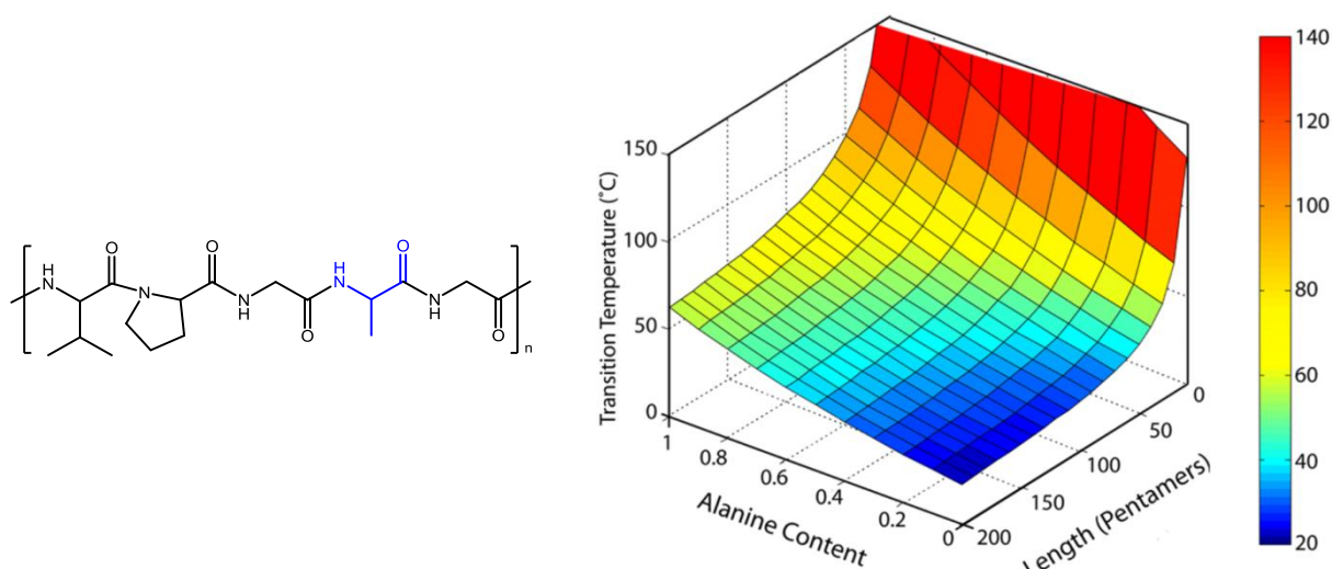
Figure 5: Left: Chemical structure of the pentapeptide Valine-Proline-Glycine-Alanine-Glycine [VPGAG] that is repeated to obtain the elastin-like polypeptides, with alanine (in blue) being a guest residue that can be changed to modulate the physico-chemical properties of the ELPs. Right: A 3-dimensional plot of the predicted inverse transition temperature T_t landscape for the alanine and valine superfamily of ELPs at 25 \mu M in PBS (taken from McDaniel et al.)[45].
