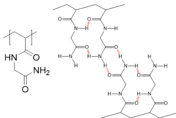
Figure 19: Left: chemical structure of poly( N -acryloylglycinamide) (PNAGA). Right: schematic representation of two PNAGA chains with possible hydrogen bonds shown in red.
