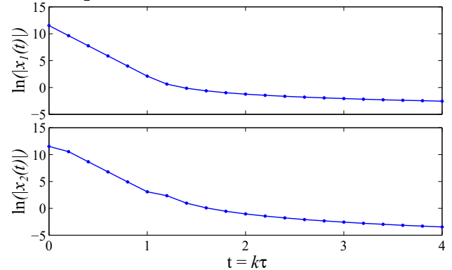
Fig. 6. States of the implicit Euler discretization of (17) with u_2 .
