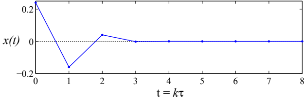
Fig. 1. State of the implicit Euler discretization of (9).
