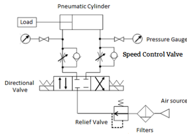
FIGURE 9. Test circuit for accelerated life test of pneumatic cylinders.
