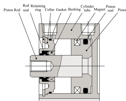
FIGURE 2. Structure of the pneumatic cylinder.
