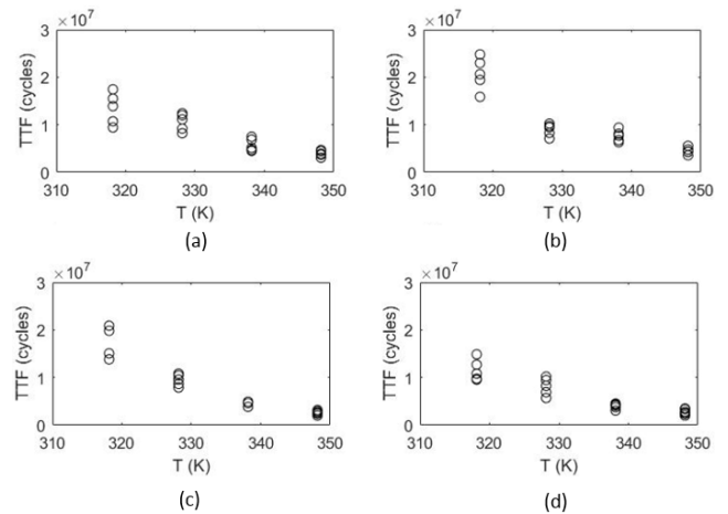
FIGURE 12. TTF data from the ALT. (a) V = 50 (cpm). (b) V = 75 (cpm). (c) V = 100 (cpm). (d) V = 125 (cpm).
