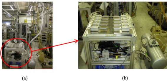
FIGURE 11. Normal life test equipment. (a) Test bench of conventional life testing. (b) Samples for conventional life testing.
