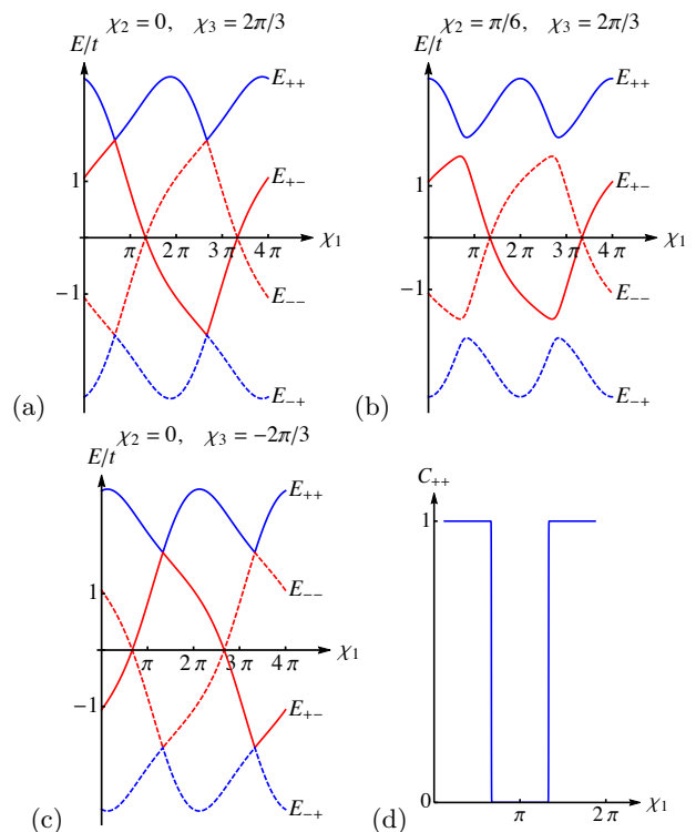
FIG. 2: Phase dependence of (a)-(c) the Andreev spectrum and (d) the Chern number in a symmetric four-terminal tunnel junction with t'/t = 0.2 and \phi = 4\pi/3 .
