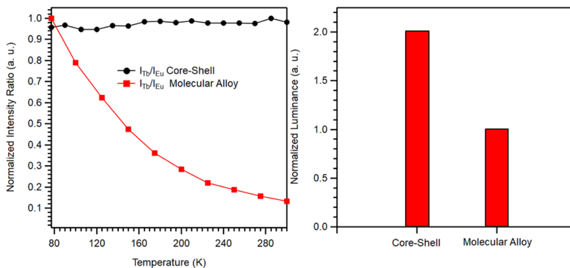
Figure 8. Left: I_{Tb}/I_{Eu} vs T have been drawn for ([Tb(cpboH)]_{\infty})_{0.5}@([Eu(cpboH)]_{\infty})_{0.5} and [Tb_{0.5}Eu_{0.5}(cpboH)]_{\infty} ( I_{Ln} symbolizes integrated intensity of the major emission peak of a Ln^{3+} ion ( {}^5D_4 \rightarrow {}^7F_5 centered at 545 nm for Tb^{3+} and {}^5D_0 \rightarrow {}^7F_2 centered at 612 nm for Eu^{3+} ) with \lambda_{exc} = 303 nm). Right: Normalized luminance of ([Tb(cpboH)]_{\infty})_{0.5}@([Eu(cpboH)]_{\infty})_{0.5} and of [Tb_{0.5}Eu_{0.5}(cpboH)]_{\infty} under UV irradiation ( \lambda_{exc} = 312 nm).
