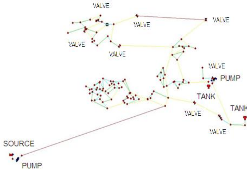
Figure 3. A WDN layout (BWSN) with 126 nodes, 1 source, 2 tanks, 168 pipes, 2 pumps, 8 valves [5]
