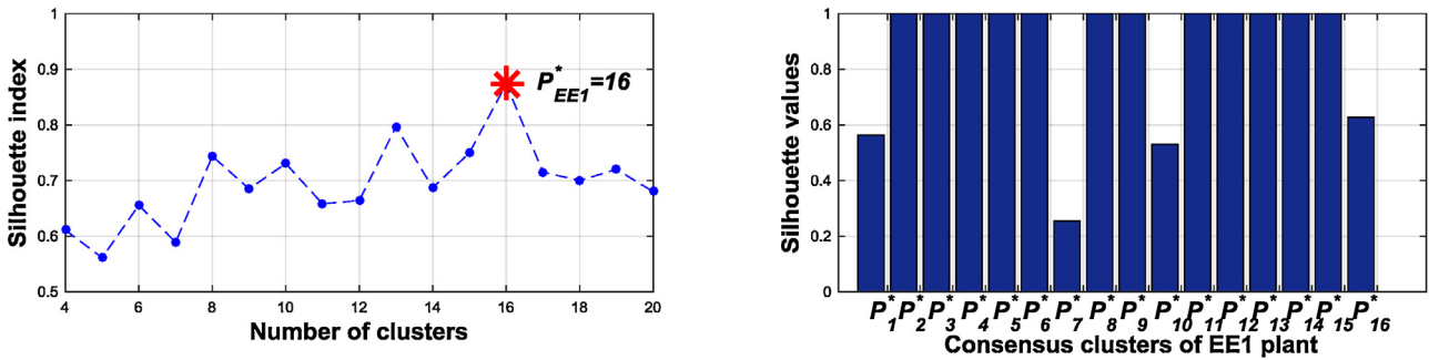
Fig. 8. Silhouette values vs. cluster numbers (left) and the individual Silhouette values of each consensus cluster obtained for the optimum number of clusters (right).
