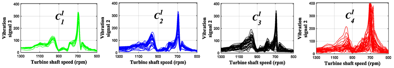
Fig. 6. Evolution of vibration signal 2 of the 4 clusters ( C_1^I , C_2^I , C_3^I and C_4^I ) of the j=1 base clustering and the corresponding turbine shaft speed values of EE1 NPP turbine.
