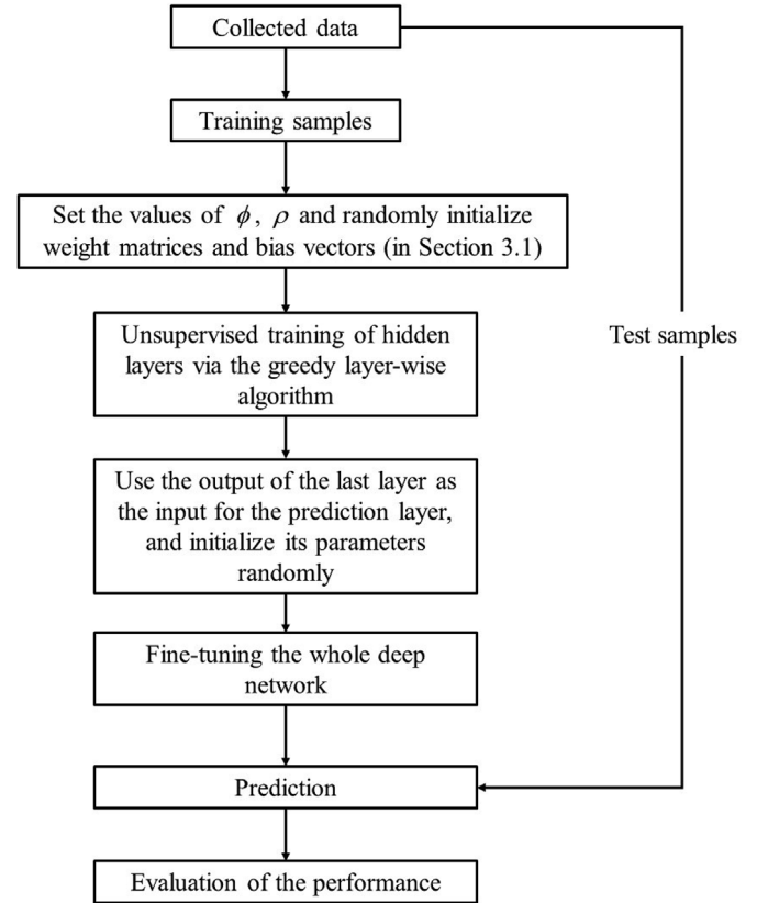
Fig. 3. The flowchart of the training process.
