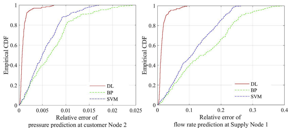
Fig. 11. Performance comparison based on the empirical CDF of the relative error of prediction results (9h prediction).
