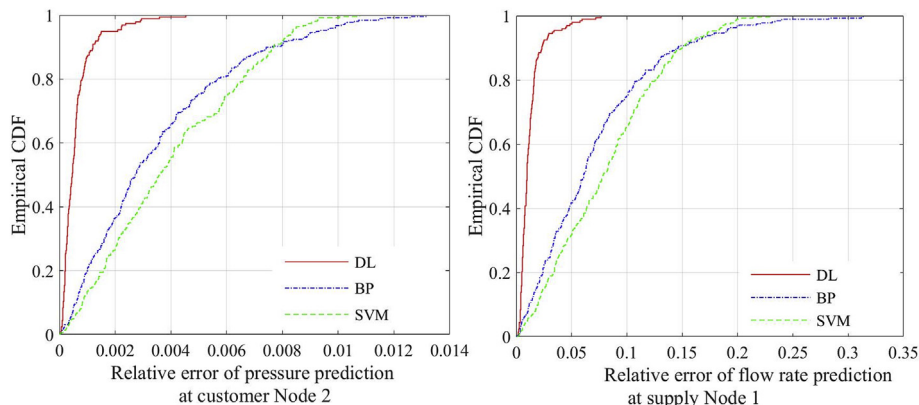
Fig. 9. Performance comparison based on the empirical CDF of the relative error of prediction results (3 h prediction).
