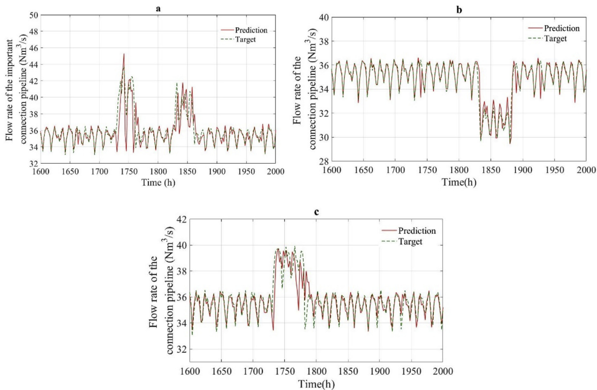
Fig. 20. Predictions of the flow rate of connection pipeline (Scenarios 1–3): Fig. a represents the results in Scenario 1; Fig. b represents the results in Scenario 2; Fig. c represents the results in Scenario 3.
