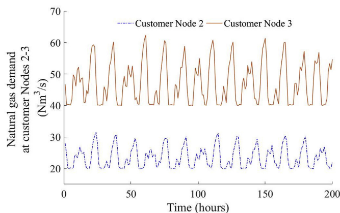
Fig. 8. The generated demands at customer Nodes 2–3 (0–200 h).
