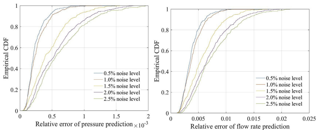
Fig. 15. Performances comparison based on the empirical CDFs of the relative error values of the predictions, based on under different levels of noises.
