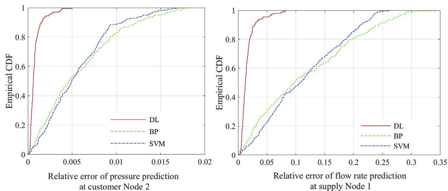
Fig. 10. Performance comparison based on the empirical CDF of the relative error of prediction results (5h prediction).
