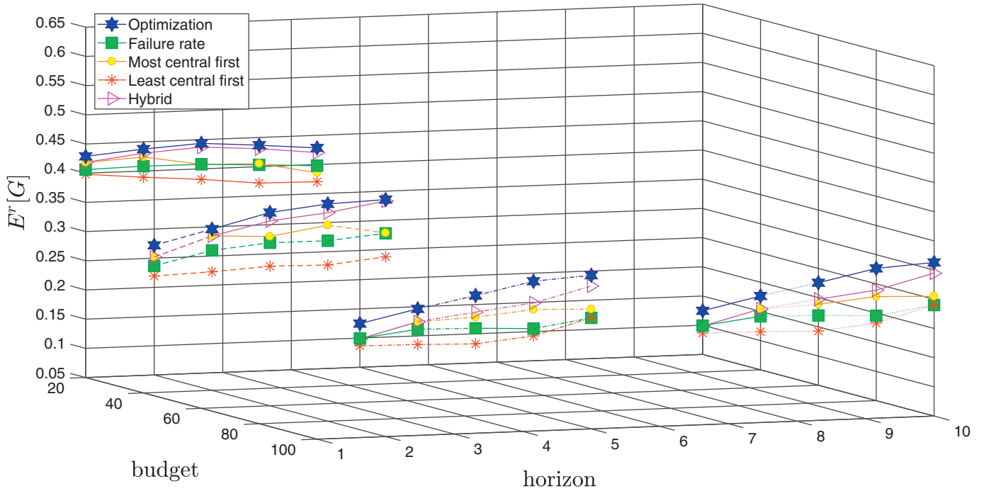
Fig. 13. Comparison of PDA with intuitive approaches.
