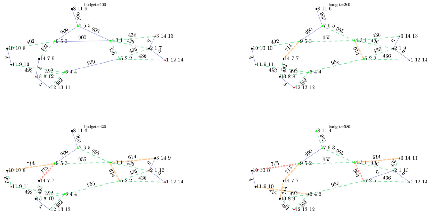
Fig. 12. Network graphs corresponding to the optimal solutions at budget levels 100,260,420,580, T = 10 . Edges where a = \emptyset are indicated by continuous lines, those with a = L_1 by dashed lines, a = L_2 by dashed-dotted lines and a = L_3 by dotted lines.
