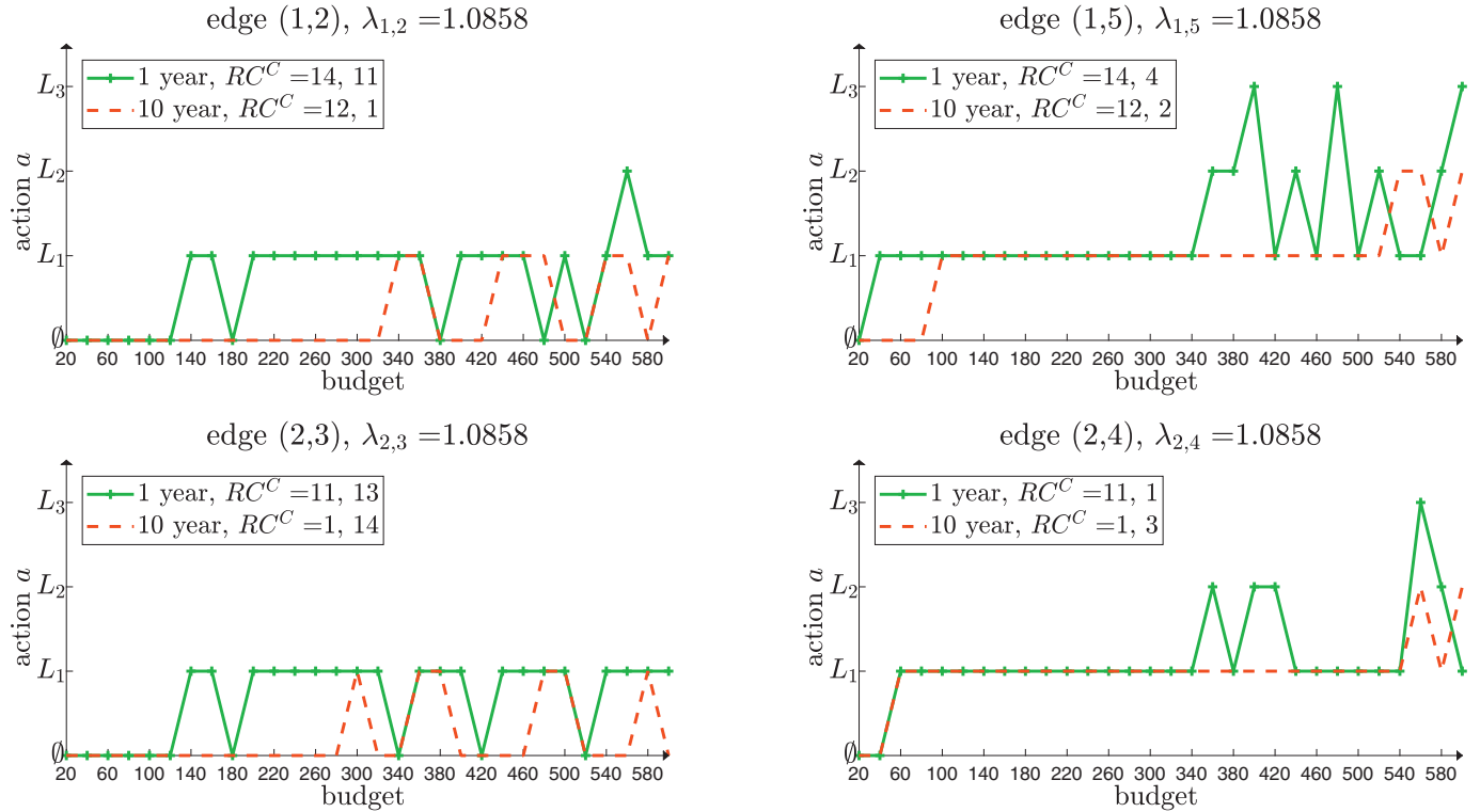
Fig. 6. Action a vs budget for edges 1–4.
