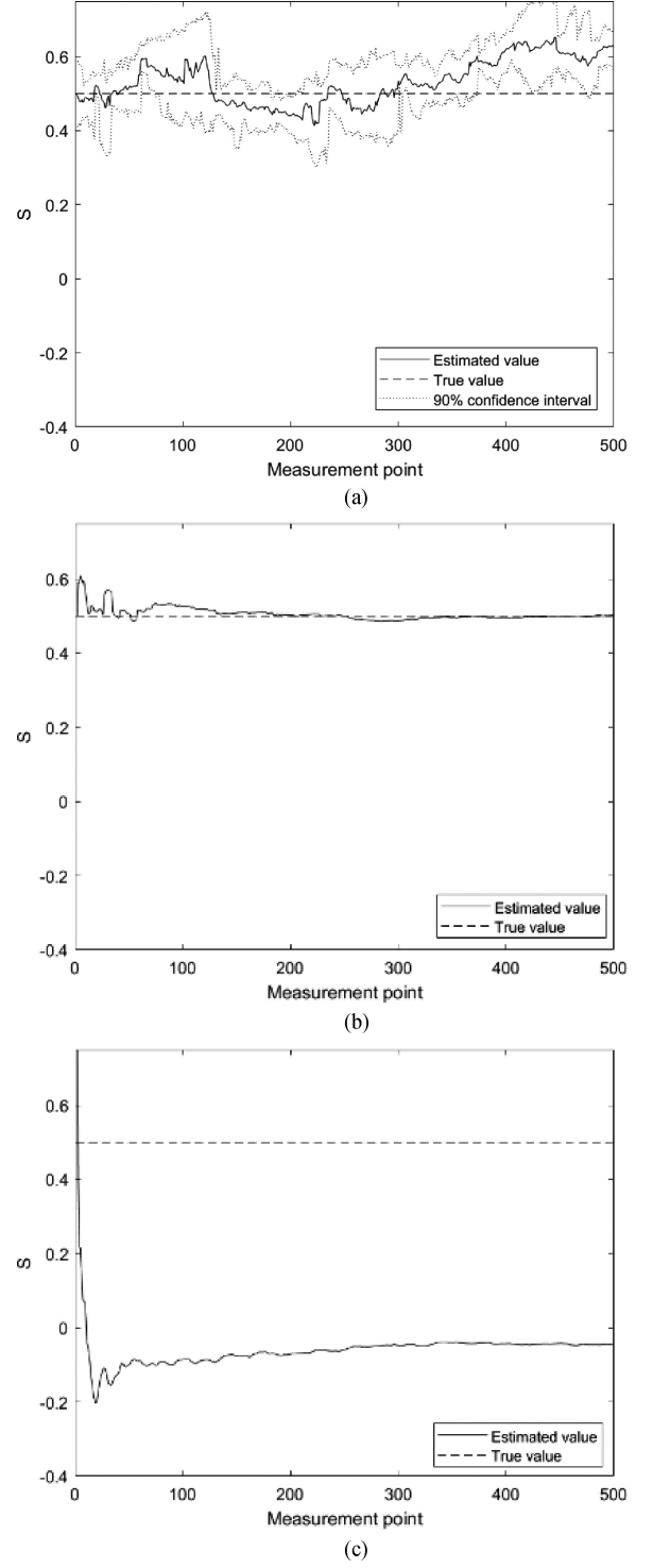
Fig. 5. Estimates of the shock damage. (a) The developed model. (b) Ke's model with accurate shock records. (c) Ke's model with imprecise shock records, error rate q = 70\% .
