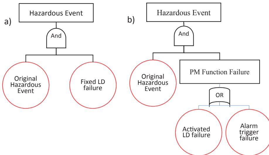
Fig. 3. Fixed devices (a) and activated devices (b).
