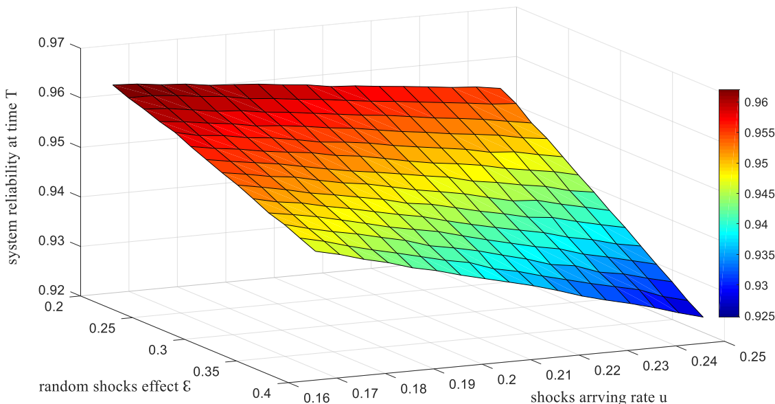
Fig. 18. The reliability of the phased AOCS with and without random shocks for different combinations of u and \varepsilon .
