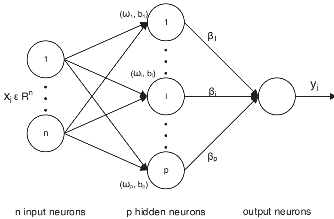
Fig. 2. Extreme learning machine model topography.
