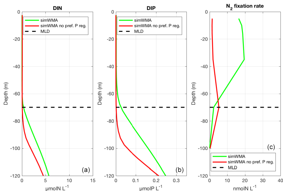
Figure 5. Vertical profiles of (a) dissolved inorganic nitrogen (DIN), (b) dissolved inorganic phosphorus (DIP), and (c) \text{N}_2 fixation rates for the simulation with diazotrophy, as a proxy of the WMA region ( \text{sim}^{\text{WMA}} ) with the preferential P regeneration (in green) and without the preferential P regeneration (in red). The horizontal black dashed line represents the depth of the maximum mixed layer calculated at 70 m depth.
