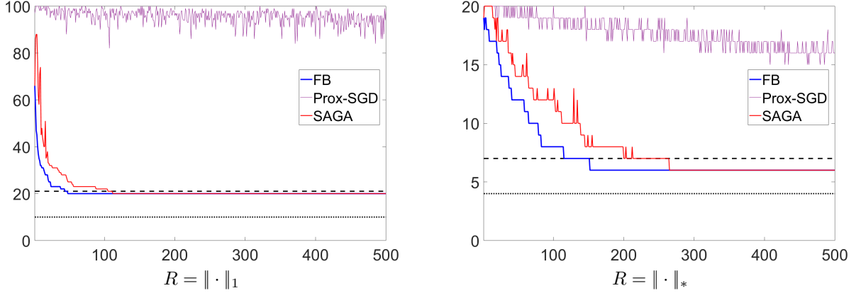
Figure 1: Evolution of R_0(M_{\hat{w}^k}) along the batches of the FB (blue), Prox-SGD (purple) and SAGA (red) algorithms, applied to solve (P_{\lambda,n}) . The black dotted line (resp. black dashed line) indicates the value R_0(M_{w_0}) (resp. the value of R_0(\mathcal{J}_{R^*}(M_{\eta_0}^*)) ); these are the dimensions of the two extreme strata.
