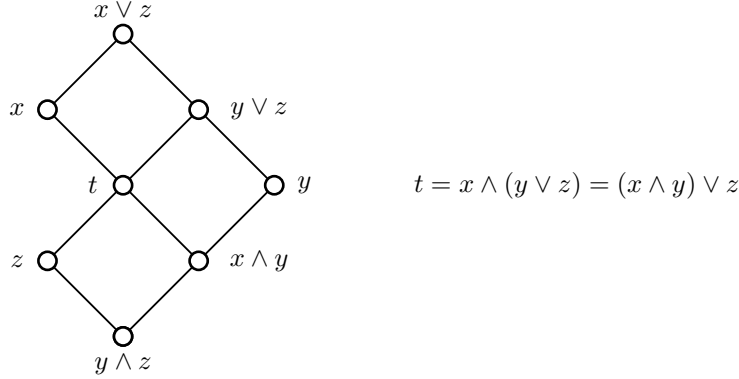
FIGURE 5.1. Illustrating the proof of (Cev3) in any \ell -group
