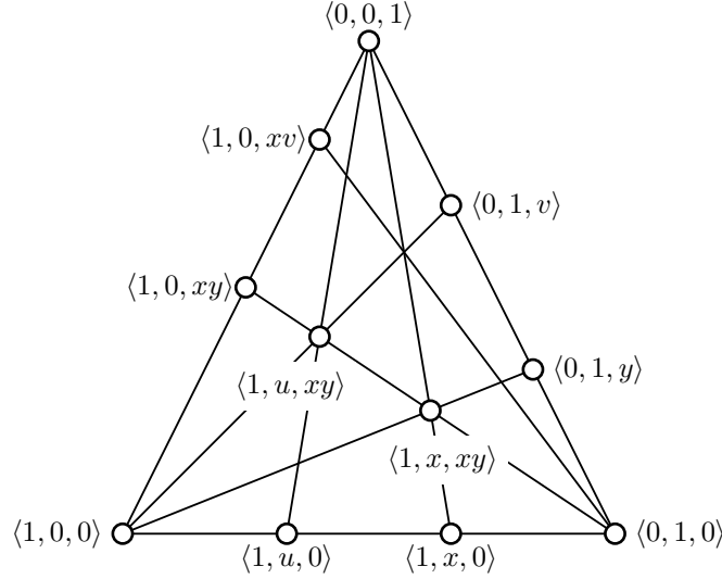
FIGURE 3.3. Illustrating the proof of Proposition 3.1, Claim 1
