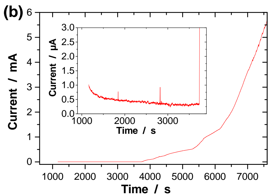
Fig. 8. Time records of the current fluctuations when the SS WE was polarized at 200 mV vs. SCE at time 0: (a) in the lab-gel cell ( f_s = 100 Hz); (b) in the portable-gel cell ( f_s = 1 Hz).
