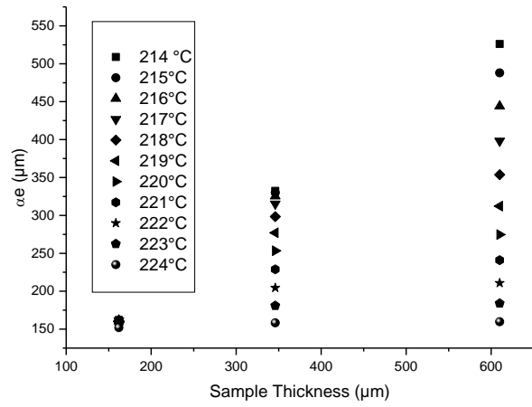
FIGURE 14 Determination of bulk crystallization at a cooling rate of 10^\circ\text{C}/\text{min} : \alpha_e vs. sample thickness for temperatures ranging from 214 to 224^\circ\text{C}
