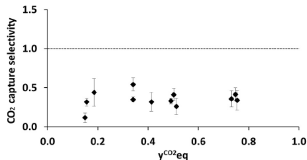
Fig. 6. CO 2 capture selectivity at equilibrium versus the equilibrium CO 2 mole fraction in the gas phase.
