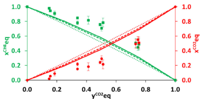
Fig. 5. Clathrate composition in CO 2 (red) and CH 4 (green) at the equilibrium clathrate forming conditions as a function of the equilibrium CO 2 mole fraction in the gas phase. Experimental data: (●) CO 2 and (■) CH 4 . Modeled data using the Conde et al. model [11]: (solid line) 344 K, (dashed line) 325 K and (dotted line) 298 K. (For interpretation of the references to color in this figure legend, the reader is referred to the web version of this article.)
