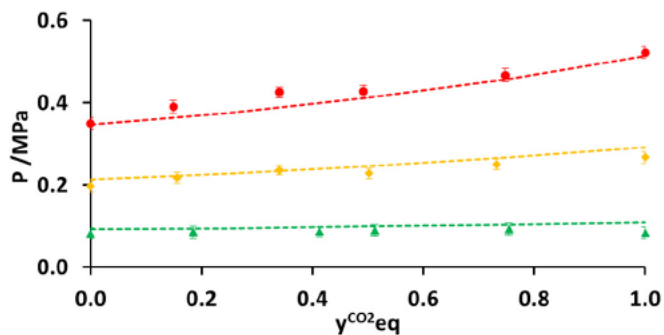
Fig. 4. Clathrate equilibrium pressure as a function of the equilibrium CO 2 mole fraction in the gas phase at 344 K (red), 325 K (yellow) and 298 K (green). Symbols: experimental data. Dashed line: modeled data using the Conde et al. model [11]. (For interpretation of the references to color in this figure legend, the reader is referred to the web version of this article.)
