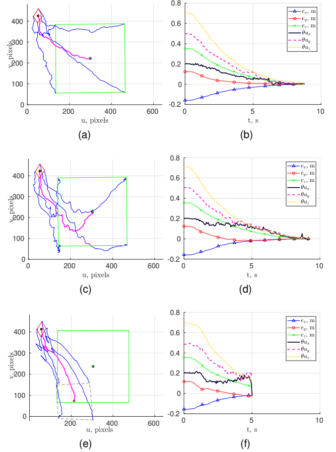
Fig. 9. CDP behavior depending on added perturbations. (a) and (b): the AprilTag trajectory and error e over time for the “base” case; system is stable. (c) and (d): the AprilTag trajectory and error e over time when tolerable perturbations are added; system is stable. (e) and (f): the AprilTag trajectory and error e over time when significant perturbations out of bounds of stability are added; system is not stable.
