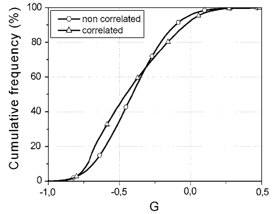
Fig. 12 Cumulative distribution function of the performance function G under loading conditions for which V_r and \alpha_r are the only random variables
