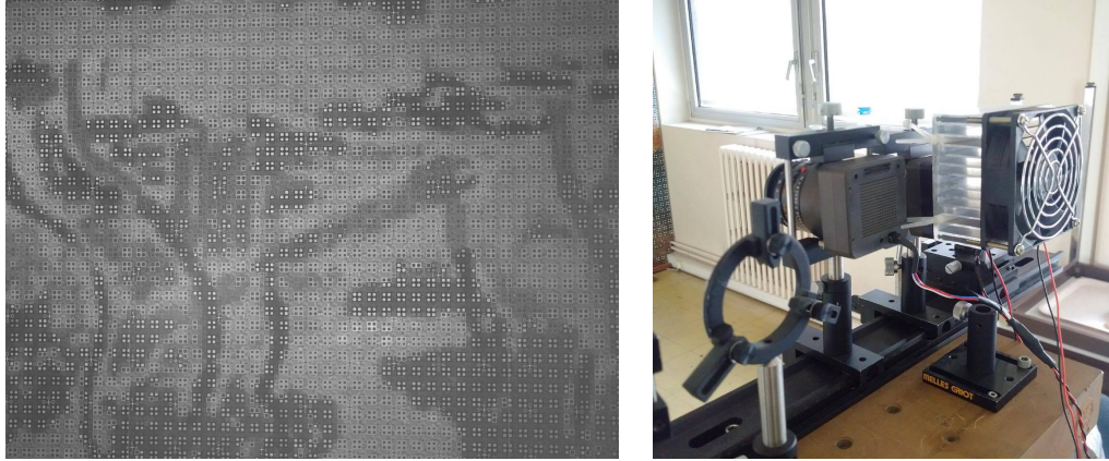
FIGURE 3: The scene of the textured wall (left) and the installation of cameras and Peltier cooler (right).
