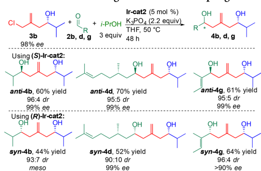
Scheme 3. Diastereodivergent Reductive Coupling of 3b
