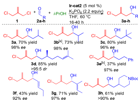
Scheme 2. Scope of the Ir-cat2 Condensation of 1 with 2a-h
