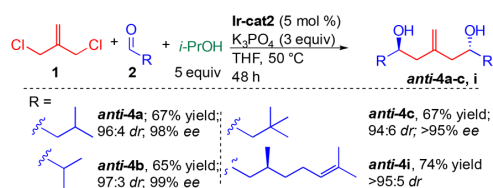
Scheme 4. Cascade Bidirectional Reductive Coupling of 1
