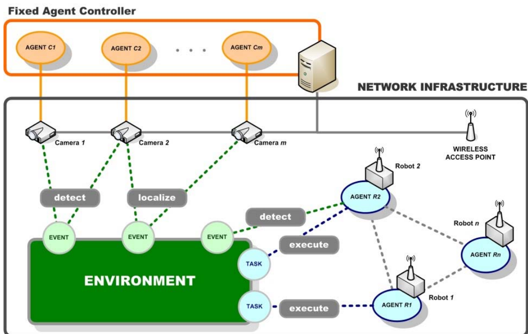
Fig. 79 - Architecture of the surveillance system
