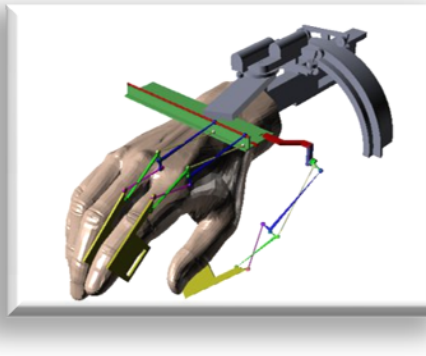
Fig. 31 - Hand active orthosis for the rehabilitation of motor functions at the GRAP
