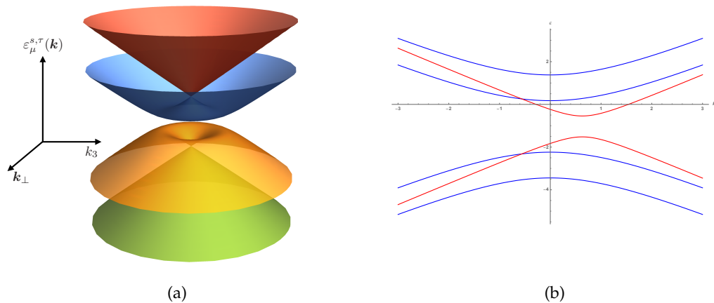
Figure 1. (color online) (a) Band structure of \mathcal{H} at zero magnetic field but finite chemical potential. Contrary to Hermitian systems, the presence of chemical potentials might modify strongly the spectrum. (b) Landau level spectrum for the non-Hermitian model for finite chemical potential \mu . Finite values of \mu shifts the LLL spectrum (red) not only upwards or downwards, but it is laterally shifted. The lateral shift makes the contribution from LLL to be non-zero for the CME.
