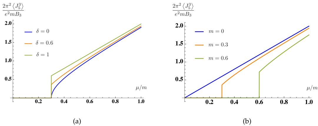
Figure 3. (color online) (a): Regularized CSE as a function of \mu for three values of \delta = m_5/m . We fix the mass parameter to be m = 0.3 . (b): CSE as a function of \mu for three values of m and fixed \delta = 0.6 .
