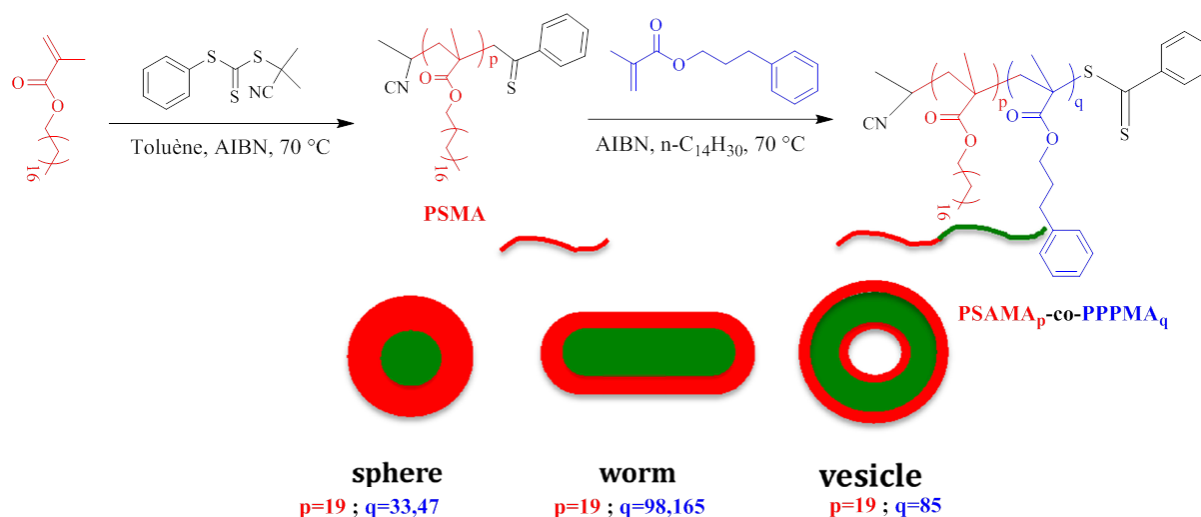
Scheme 11: Synthesis of \text{PSMA}_p\text{-co-PPPMA}_q copolymer nanoparticles via RAFT dispersion in n-tetradecane at 70 °C
