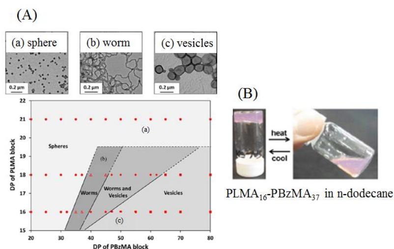
Figure 13: (A) Phase diagram constructed for PLMA x -PBzMA y diblock copolymer nanoparticles prepared by RAFT dispersion polymerization of BzMA in n-dodecane at 20% w/w solids (B)Thermo-responsive solution behavior exhibited by 20% w/w PLMA 16 -PBzMA 37 diblock copolymer nanoparticles in n-dodecane.
