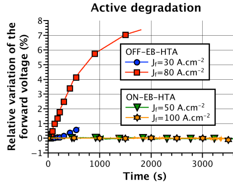
Fig. 8: Active degradation measurements made on OFF-EB-HTA and ON-EB-HTA .
