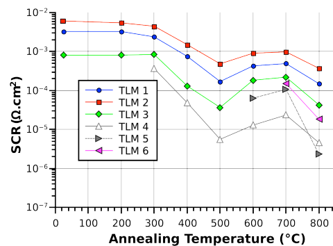
Fig. 2: Evolution of the SCR as a function of the annealing temperature for six different TLM patterns at different places on the sample.
