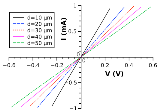
Fig. 1: I-V plots as a function of the spacing distance between pads of a typical TLM pattern on non-annealed VLS grown p + doped island
