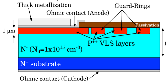
Fig. 5: Cross section view of the fabricated diodes.
