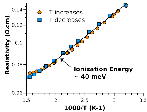
Fig. 4: Arrhenius plot of the VLS layer resistivity.
