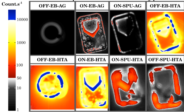
Fig. 7: PEM pictures at I=100 \text{ mA} of different processed PiN diodes.
