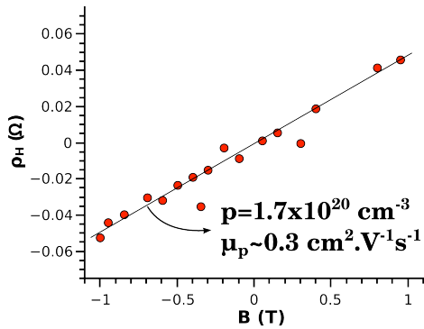
Fig. 3: Hall resistance ( \rho_H ) of the VLS layer as a function of magnetic field ( B ) at I = 1 \mu\text{A} , T = 300\text{K}
