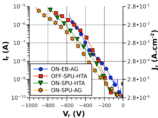
Fig. 9: Leakage current of best diode of each condition.
