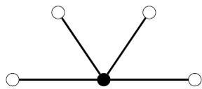
Figure 1. A Star K_{1,4} .
