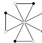
Figure 7. A friendship graph F_4 .
