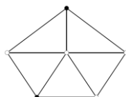
Figure 10. A wheel graph W_5 .
