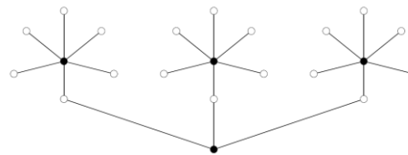
Figure 12. A banana tree B_{3,7} .
