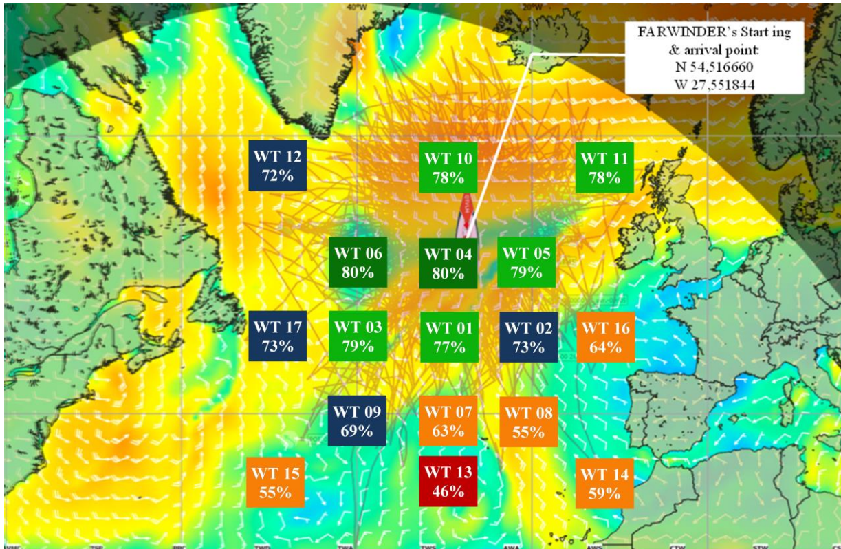
Figure 3. Tested locations for the wind turbines and average capacity factor over the three years of 2015, 2016 and 2017
