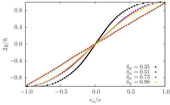
Figure 3. Velocity profiles for four different values of roughness angle \delta_w and a constant nominal inertial number I_e \approx 0.01 in the steady state, for a fixed average flow thickness h/d \approx 50 . Solid lines are fits by equation (6).
