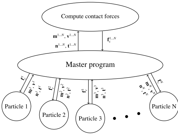
Fig. 3. Scheme of the parallelisation procedure of the MPM-CD framework; N is the number of the particles and \mathbf{f}_c , \mathbf{m} , \mathbf{n} and \mathbf{t} represent the contact force, mass, normal and tangential vectors, respectively, for the potential contact nodes of each particle.
