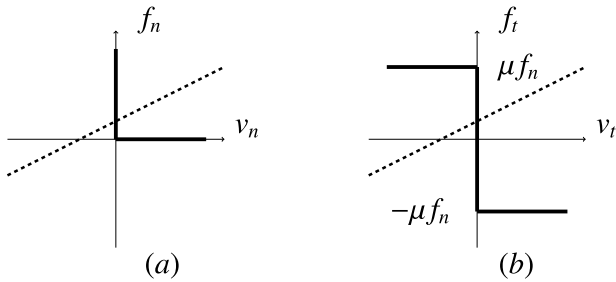
Fig. 2. Contact conditions: (a) Velocity-Signorini complementarity condition as a graph relating the normal relative velocity v_n and normal force f_n ; (b) Coulomb friction law as a graph relating the tangential velocity v_t and friction force f_t ; \mu is the coefficient of friction. The dashed lines represent the linear relations obtained from a linear combination of the equations of dynamics; see text.
