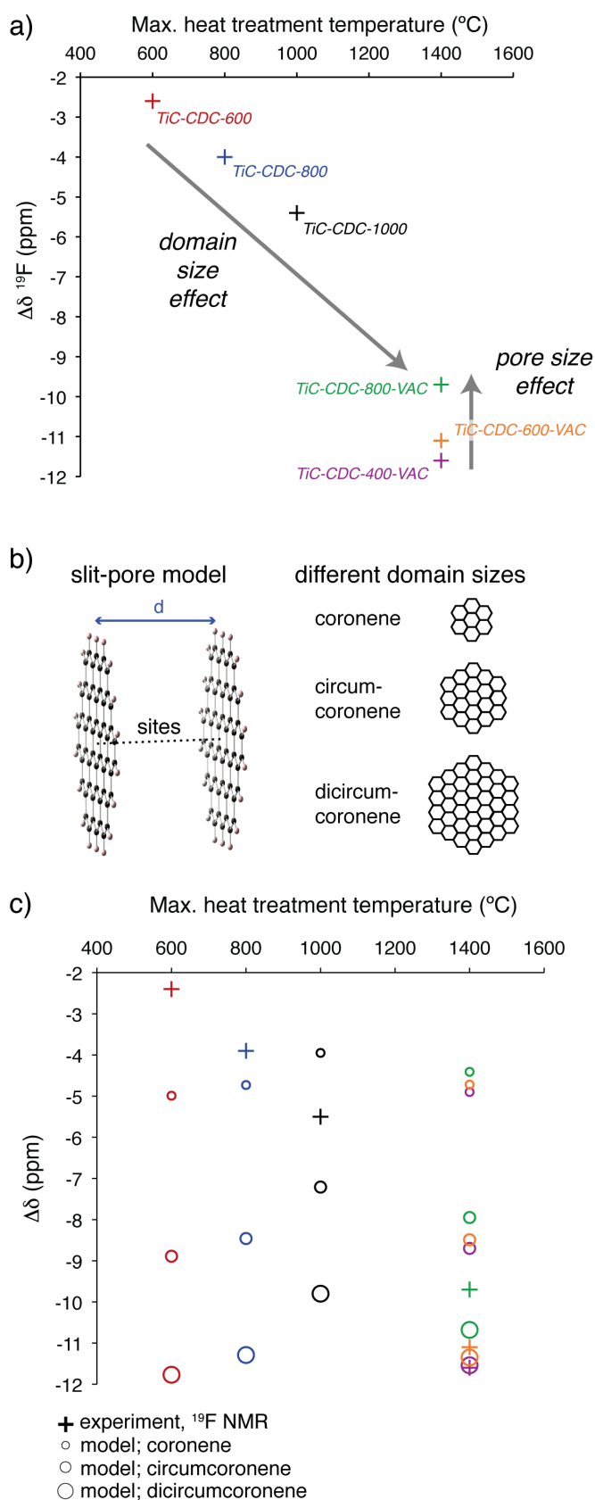
Figure 4 (a) Summary of \Delta\delta ^{19}\text{F} values measured in this work. (b) Schematic of structures used in lattice model simulations of \Delta\delta values. (c) Simulated and experimental \Delta\delta values. For each carbon, three different simulated \Delta\delta values are shown, corresponding to values computed with models employing coronenes of different sizes. The colour coding of the data points in (c) for the different carbons is given in (a).
