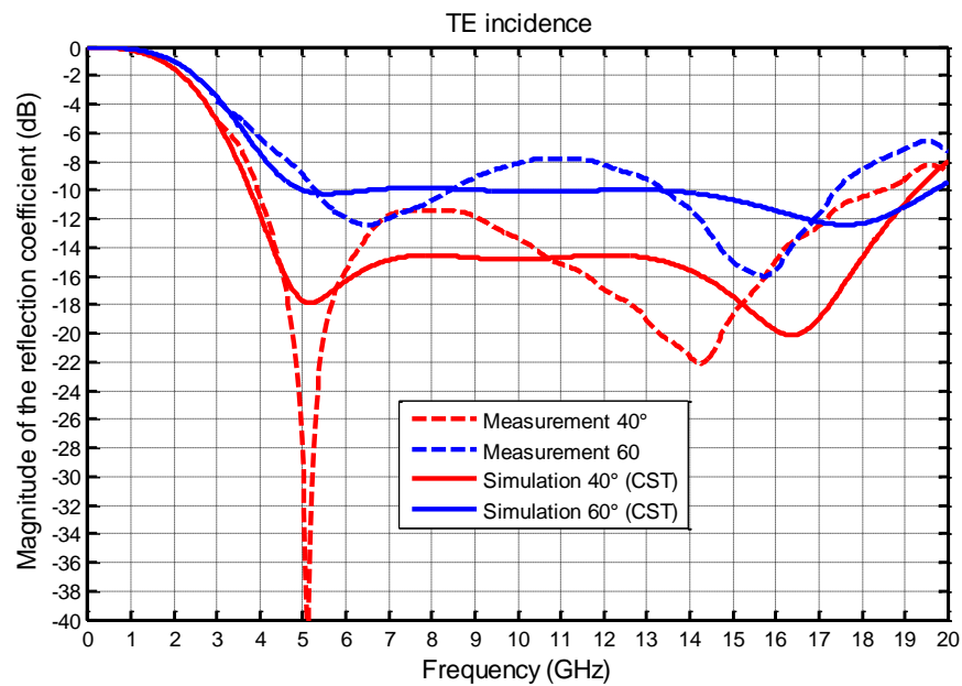
Figure 6. Comparison between the simulated and measured magnitudes of the reflection coefficient (dB) as a function of frequency with two angles of incidence 40° and 60° for TE polarization.
