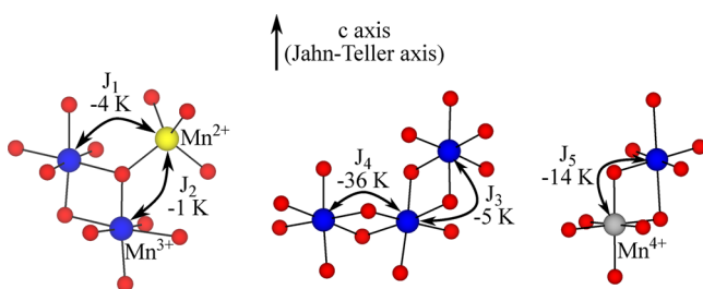
Figure 4. Mn–Mn exchange coupling constants identified in the studied systems, i.e. \text{LiTi}_{1.25}\text{Mn}_{0.75}\text{O}_4 for J_1 and J_2 , \text{LiTiMnO}_4 for J_3 and J_4 , and \text{LiTi}_{0.5}\text{Mn}_{1.5}\text{O}_4 for J_5 . For each J_n , the reported value corresponds to the average between the HYB20–HYB35 results.
