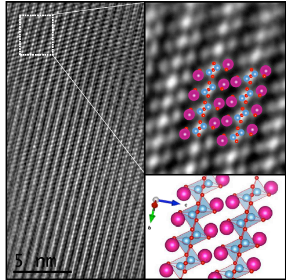
Figure 4. High resolution transmission electron microscopy image acquired on a Rb_2Ti_2O_5 sample along the [110] zone axis (HR-TEM JEM-2010F; JEOL Ltd, Tokyo, Japan). A close-up of the image is showed in the insert on which is superimposed a simulated crystal structure from X-Ray diffraction data. The Rb atoms are in pink, the Ti atoms are in blue and the O atoms are in red.
