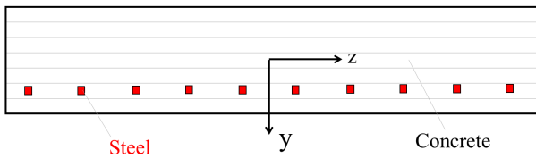
Figure 6. Cross section discretization of the beam multi fiber finite element. The diameter sizes of the steel reinforcements are knowingly exaggerated.
