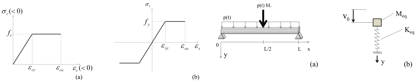
Figure 2. Stress-strain relations for concrete (a) and steel (b).
