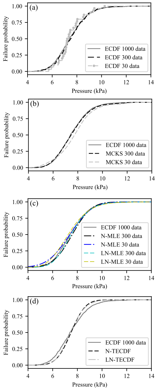
Figure 9. Reliability method comparisons between empirical cumulative distribution functions (ECDF) with set (1, \alpha) sample of size 1000 and (a) empirical cumulative distribution functions with samples of sizes 30 and 300; (b) Gaussian kernel smoothing (MCKS) cumulative distributions functions with samples of sizes 30 and 300; (c) maximum likelihood estimation cumulative distribution function (MLECDF) fitting of normal (N-MLE) and log-normal (LN-MLE) distributions with samples of sizes 30 and 300; (d) Taylor expansion of the first two centered statistical moments estimates to build normal (N-TE) and log-normal (LN-TE) cumulative distributions functions.
