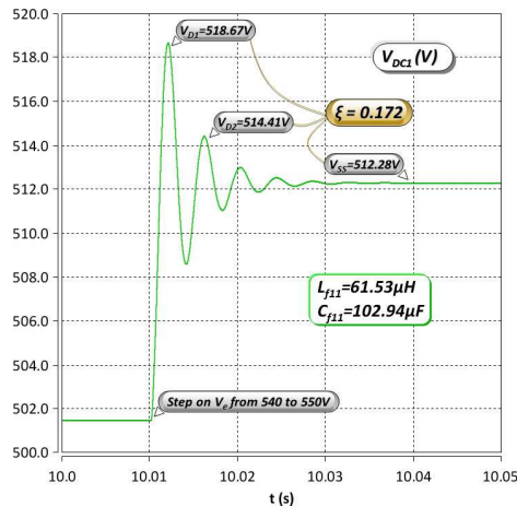
(a) Load n°1 + filter topology n°1 - V_{DC1}
