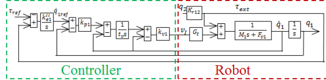
(b) Case with position loop.
