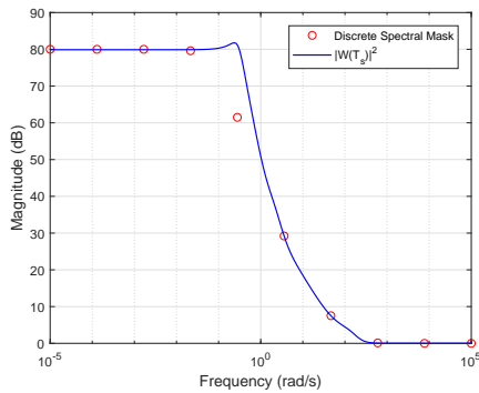
Fig. 2. H_\infty -Weights Generation Illustrative Example
