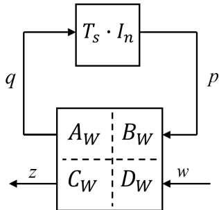
Fig. 1. Block Diagram of an identical dissipative systems interconnection
