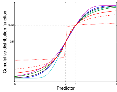
(A) F \in \mathfrak{F}_{q_{0.73}}
