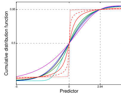
(B) F \in \mathfrak{F}_{q_{0.95}}
