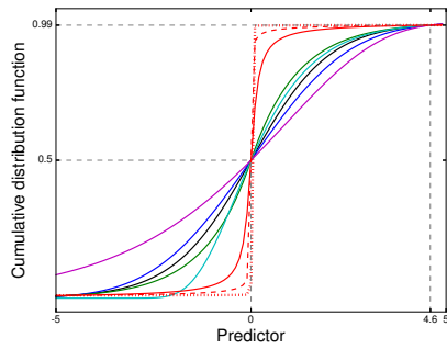
(C) F \in \mathfrak{F}_{q_{0.99}}
