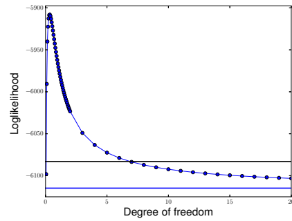
(B) (reference, Student _{\nu} , Z^{(2)} ) models
