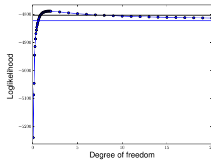
(C) (reference, Student _{\nu} , Z^{(3)} ) models
