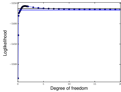
(A) (reference, Student _{\nu} , Z^{(1)} ) models
