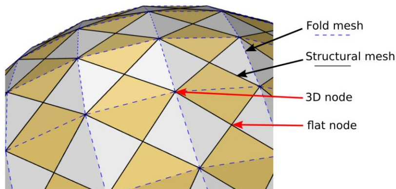
Figure 4: Fold mesh and structural mesh
