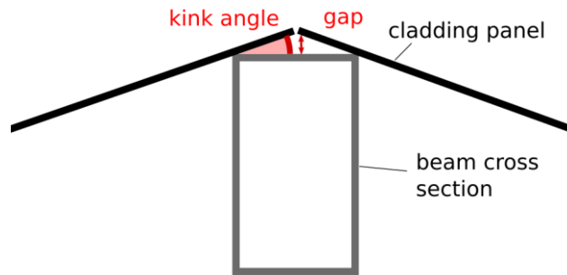
Figure 1: Kink angle between a cladding panel and a beam and corresponding gap
